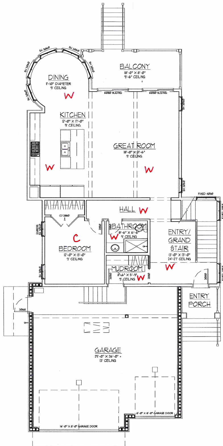
LEVEL ONE PLAN
